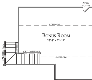
Extended Bonus Room Second Floor Option #3
